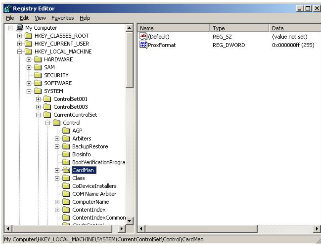
Figure 6 - Registry Editor
